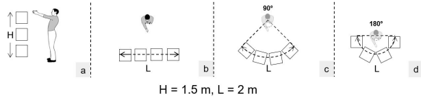
Figure 5: The shelf configuration: (a) shelf height, (b) flat shelf length, (c) quarter-circle shelf arc length, (d) half-circle shelf arc length
